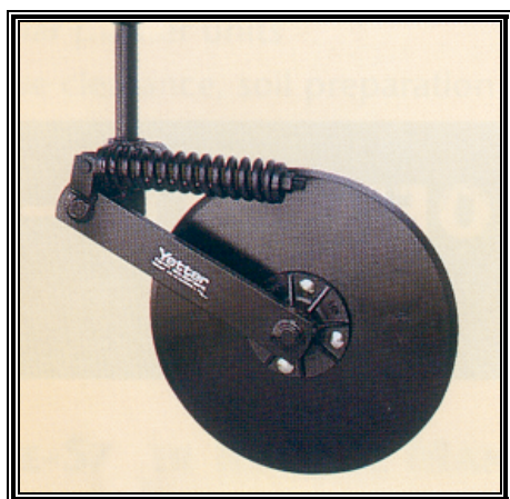
20" SMOOTH
